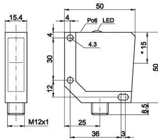
* receiver axis: 15mm
