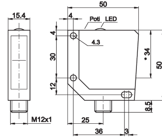
* transmitter axis: 34mm
