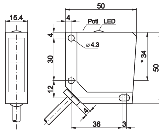
* transmitter axis: 34mm
