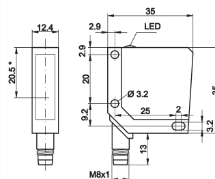
* transmitter axis: 20.5mm
