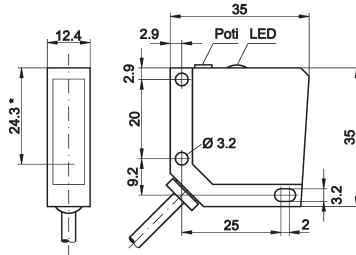
* transmitter axis: 24.3mm 24.3mm
