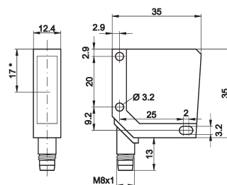
* transmitter axis: 17mm
