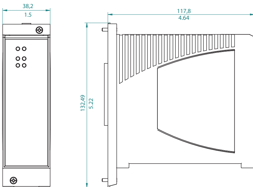
Figure 14: Dimensions for media modules with characteristic value HH
