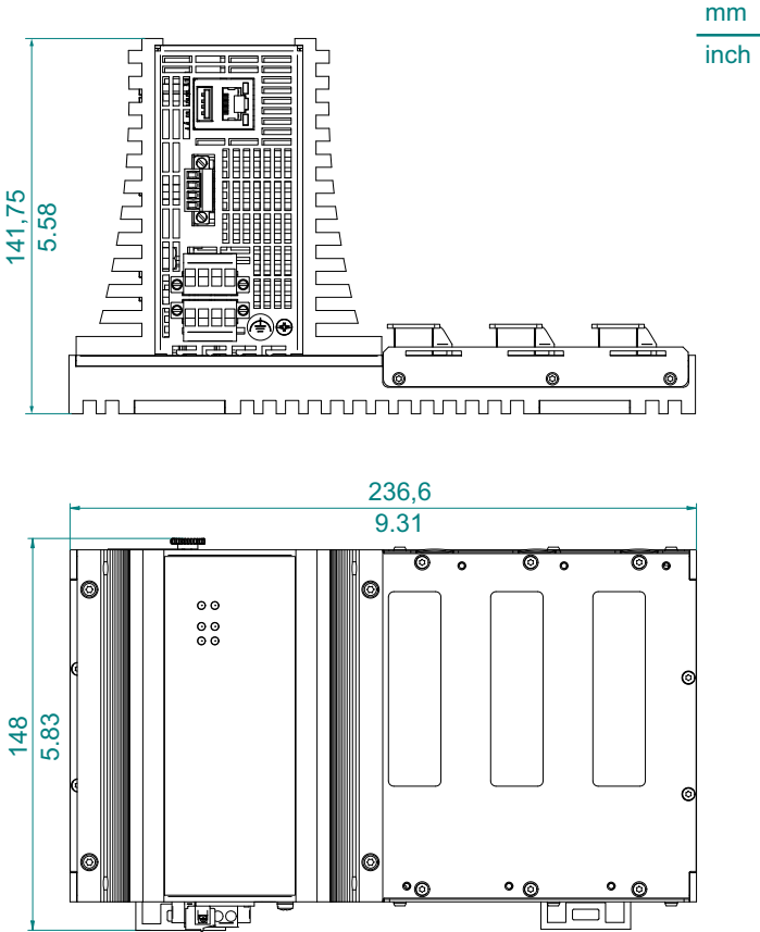
Figure 8: MSP30/32-0804.....HH..., MSP40/42-0012.....HH...
