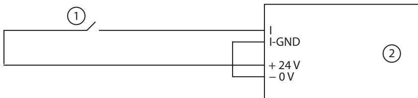
Figure 5: Circuit via auxiliary voltage supply 1 - Switch (2-wire sensor) 2 - MSM24 module
