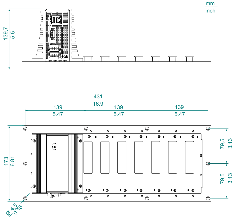
Figure 13: MSP30-2404.....HX...
