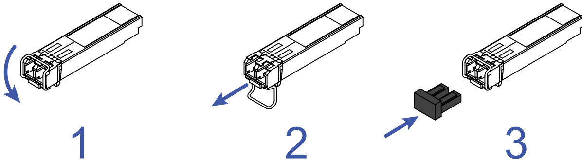
Figure 7: Removing an SFP transceiver: Removal sequence
