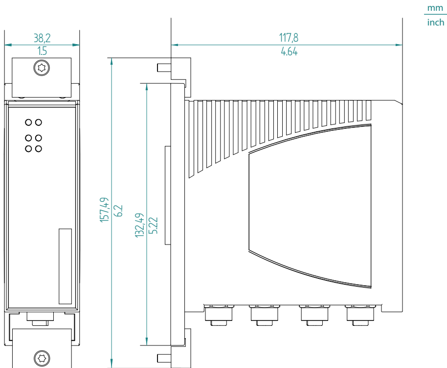
Figure 16: Dimensions for media modules with customer-specific version characteristic value HX
