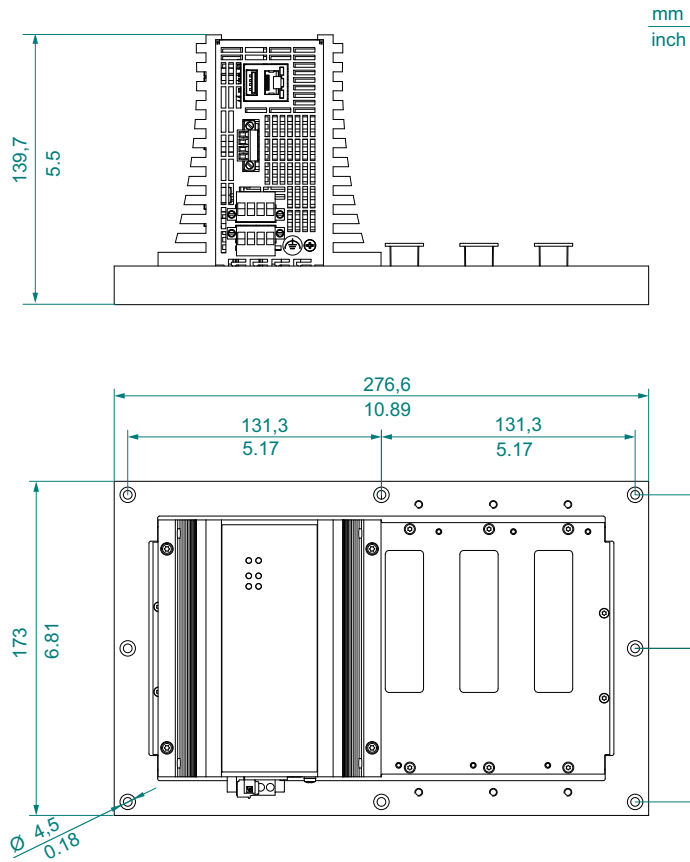
Figure 11: MSP30-0804.....HX...
