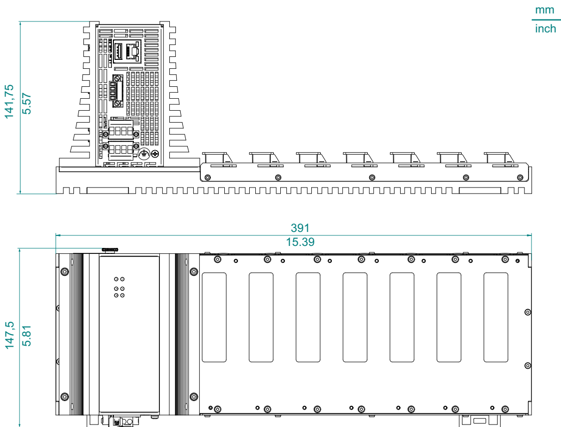
Figure 10: MSP30/32-2404.....HH..., MSP40/42-0028.....HH...
