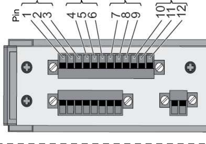
Detail of MSM24-IOIOIOIO
