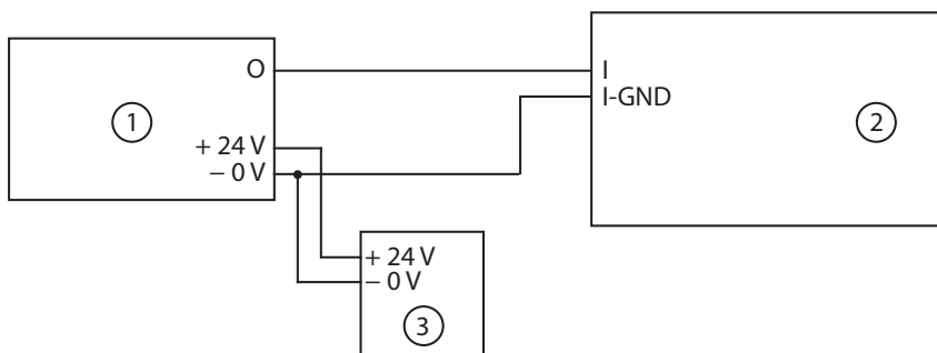
Figure 3: Connection of a sensor with separate voltage supply 1 - Sensor 2 - MSM24 module 3 - Separate voltage supply for sensor
