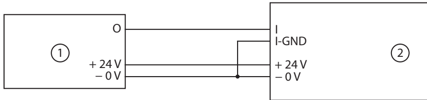
Figure 4: Connection of a sensor with auxiliary voltage supply 1 - Sensor 2 - MSM24 module
