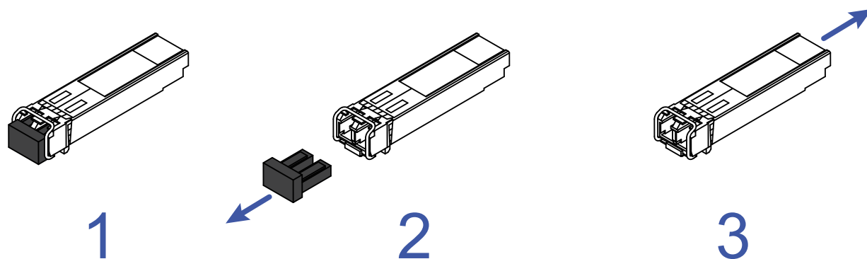
Figure 6: Installing SFP transceivers: Installation sequence
