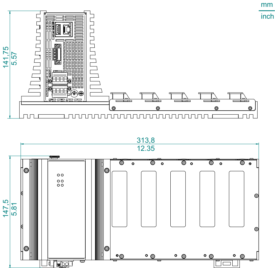
Figure 9: MSP30/32-1604.....HH..., MSP40/42-0020.....HH...
