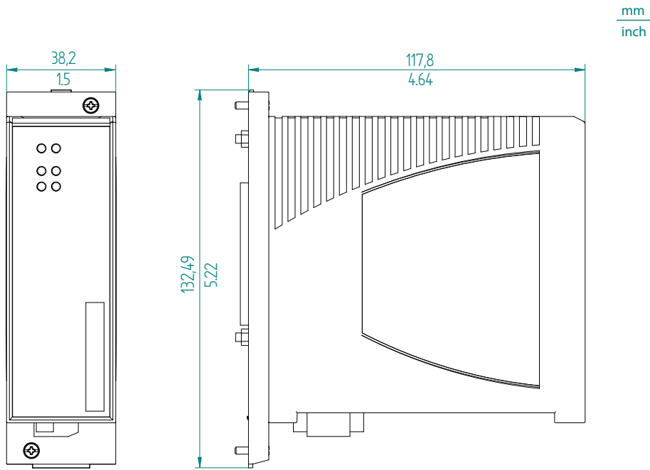
Figure 15: Dimensions for media module MSM46-T1T1T1T1... with characteristic value HH (with terminal block for external PoE supply voltage)
