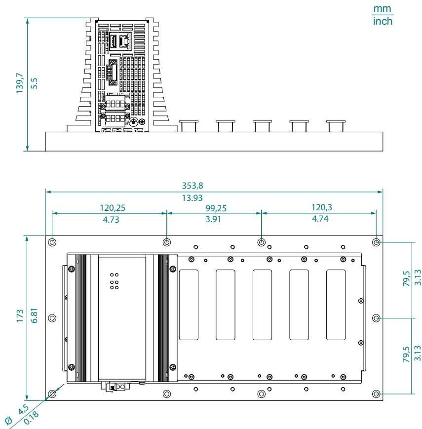
Figure 12: MSP30-1604.....HX...
