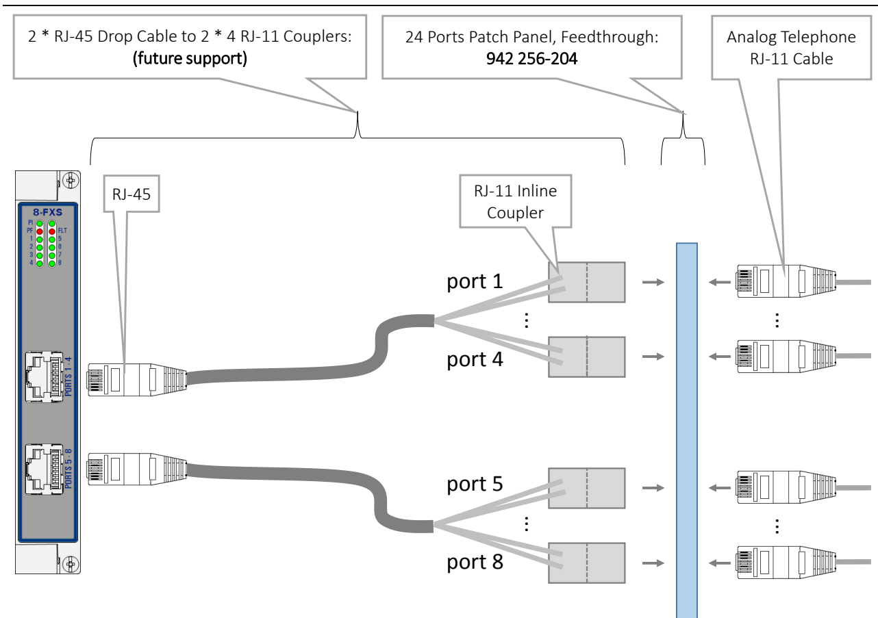
8-FXS Connection: Unplugged
