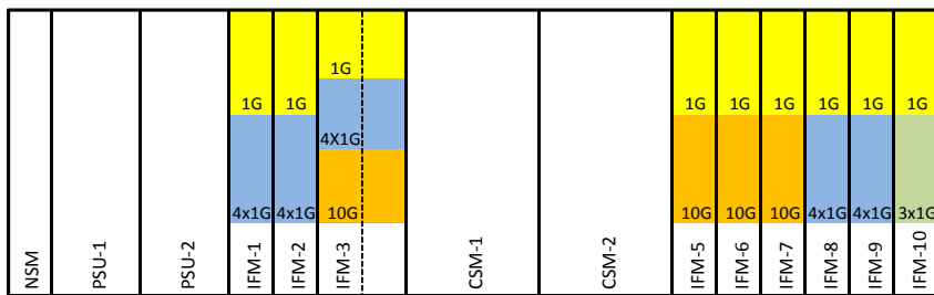
XT-2206-A: Node Slot Speeds
