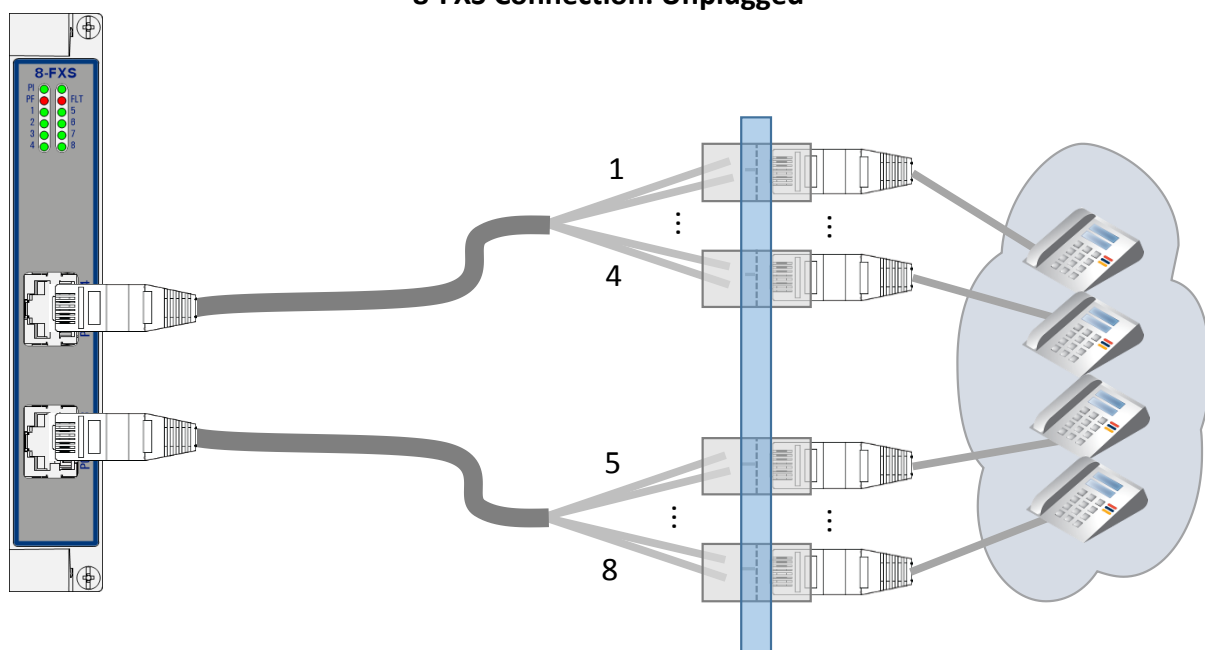
8-FXS Connection: Plugged
