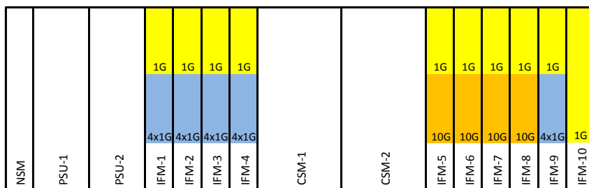
XT-2209-A: Node Slot Speeds
