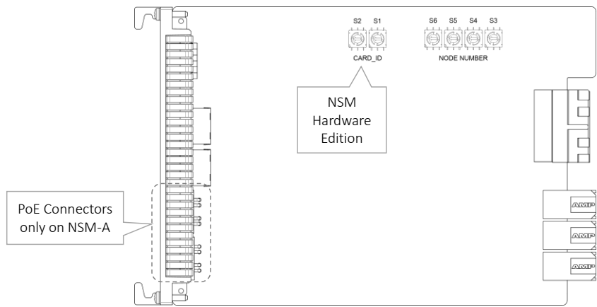
NSM-A Side view
