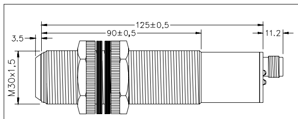
Dimensions/Abmessungen/Dimensions
